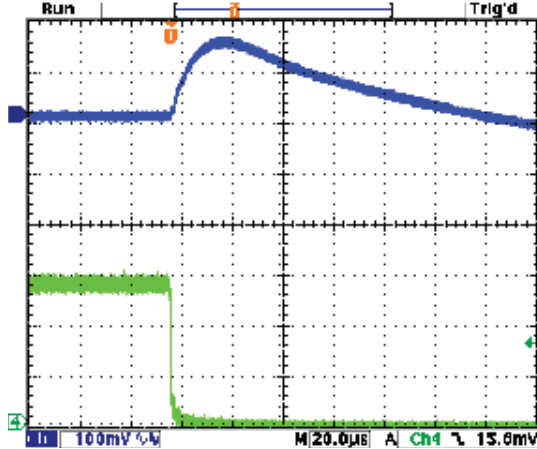
Step Load Transient Response (Vin=12V, Vout=1.8V, Cload=10x10µF X5R 0805 ceramic, plus 1x470µF, 7mΩ POSCAP, total 570µF, Iout=0A to 1.5A) Top trace=Vout, Bottom trace=Iout
